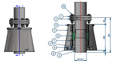
Feeding Pipe Flexible Connecting
