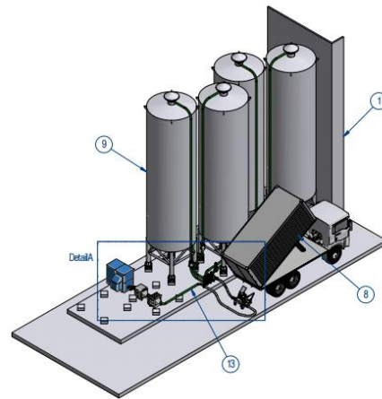
100 m 3 SUS304, PP,PE,PS & PET Storage Silos with Loading System from Container Truck
