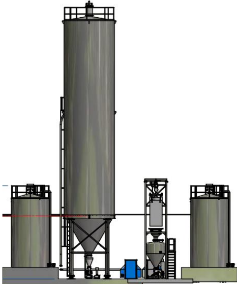
100 m 3 & 200 m 3 SUS304, PVC Storage Silos with Loading System from Bulk Truck (Tank Car) & Big Bag
