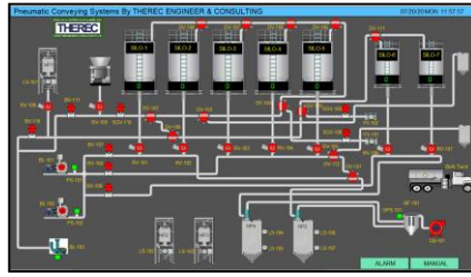
Raw Bulk & Powder Material Handling System / Control & Monitoring Computer Screen Page
