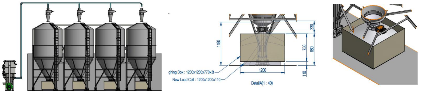
20 m 3 Plastic, PP Intermediate Silos with Shear Beam Silo Load Cell Sets and Weighing Buffer Hopper
