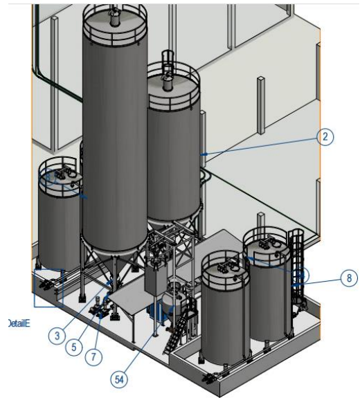
100 m 3 & 200 m 3 SUS304, PVC Storage Silos with Loading System from Bulk Truck (Tank Car) & Big Bag
