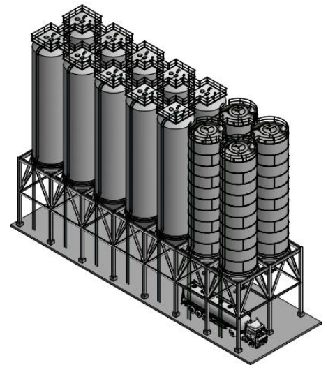
500 m 3 SUS304, PP,PE&PS Storage Silos with Loading System from Bulk Truck (Tank Car) and Unloading to the Bulk Truck, Container Truck, Big Bag or Loose Bag again for distribution
