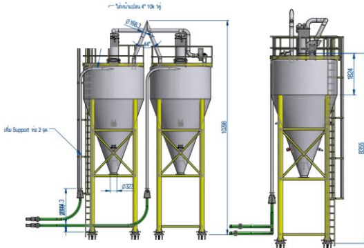
30 m 3 Stainless Steel Wheat Flour Storage Silo system
