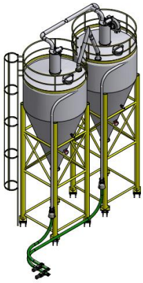
30 m 3 Stainless Steel Wheat Flour Storage Silo system
