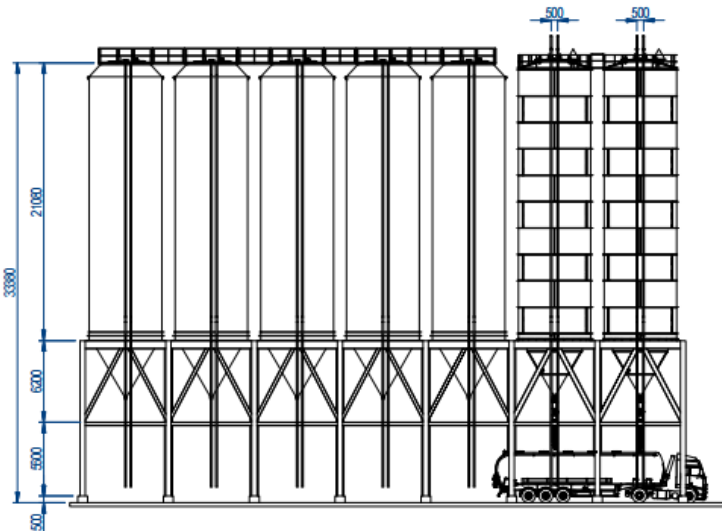
500 m 3 SUS304, PP,PE&PS Storage Silos with Loading System from Bulk Truck (Tank Car) and Unloading to the Bulk Truck, Container Truck, Big Bag or Loose Bag again for distribution
