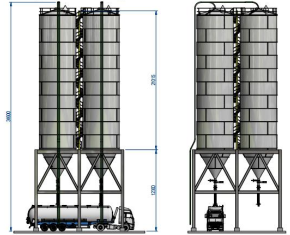
Gravity Feed Bulk Truck Loading System
