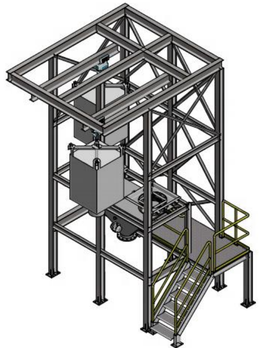
Big Bag Unloader
