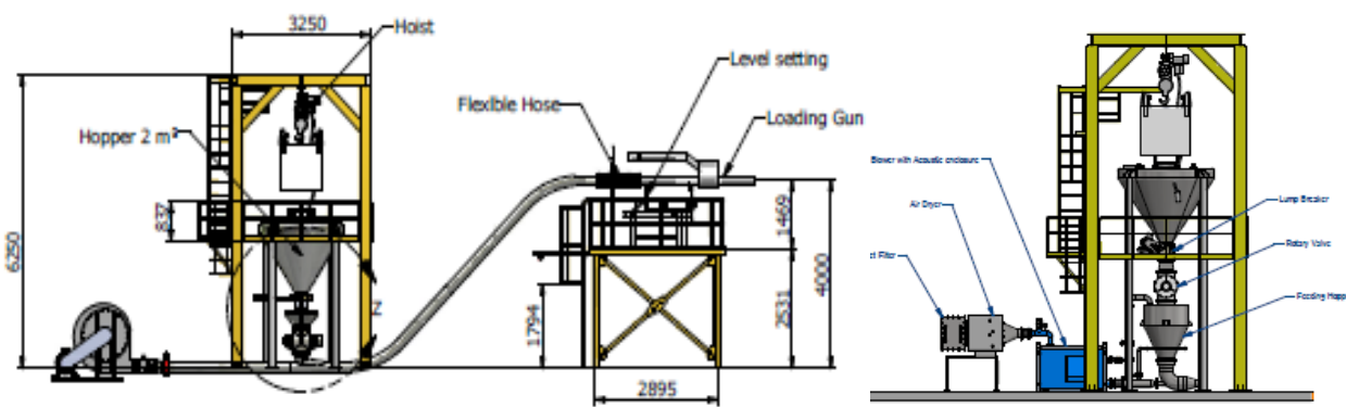
Sea bulk Loader or Bulk Truck loader / Mobile or Fixed Station
