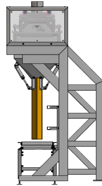
25 kg Bag Filling Machine
