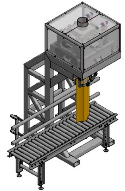
25 kg Bag Filling Machine
