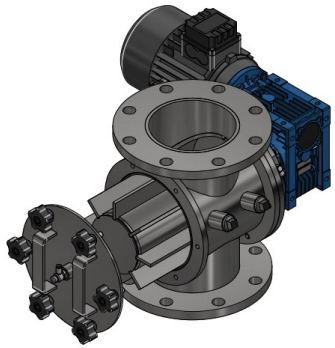
Air Lock Rotary Valve, Compact Dosing & Weighting Type, Easy Clean Series
