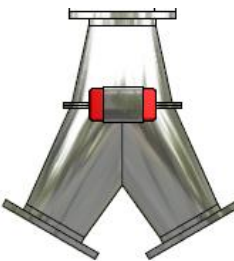
Air lock Diverter Valve
