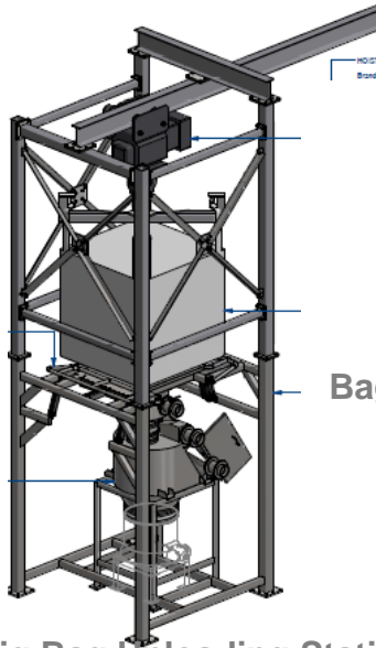
Big Bag Unloading Station
