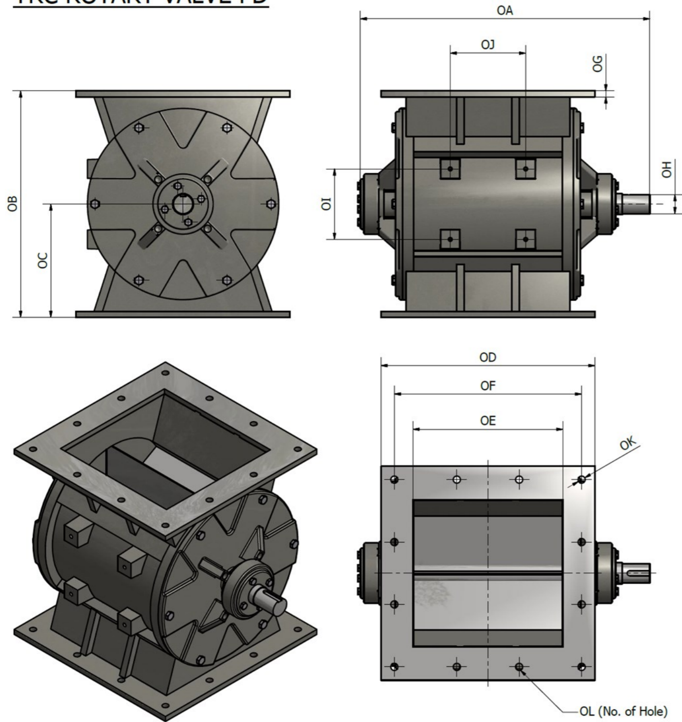
DIMENSIONS (all in millimetres)
